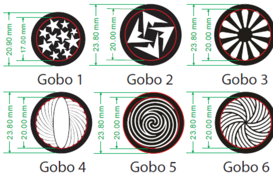
Gobo Wheel 2
